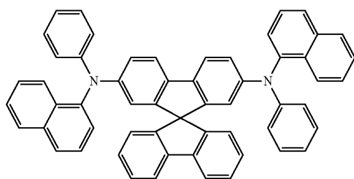
Spiro-NPB
