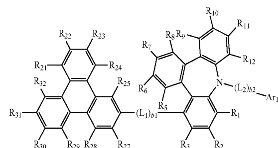
<Formula 1D>
