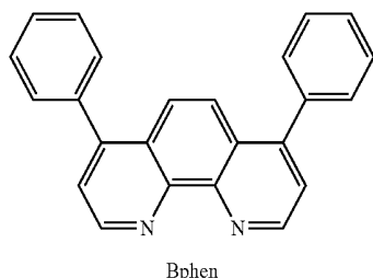
Bphen
